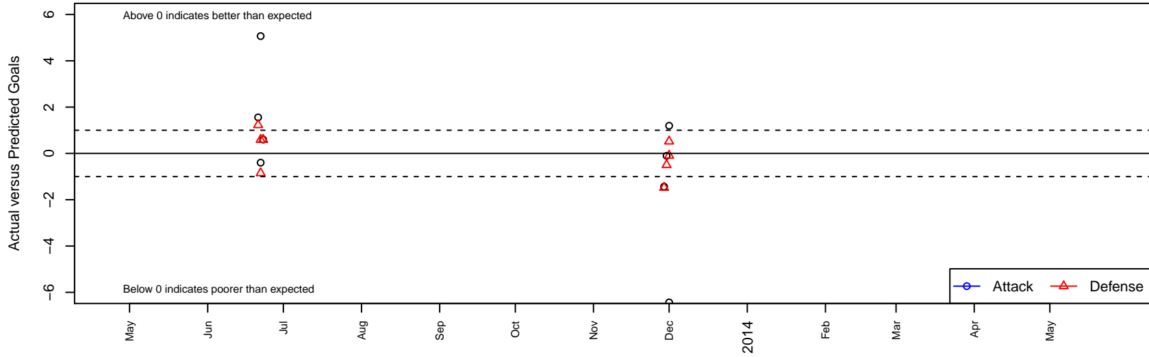
Footskills Impact G02 Dots are actual minus expected GF (blue circles) and GA (red triangles). Blue line is smoothed change in attack strength. Red is smoothed change in defense strength.
